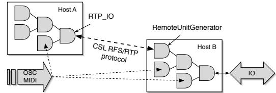
Figure 6: A multi-host CSL graph with UnitGenerator graphs running on 2 computers and a sample streaming mechanism using the RTP protocol between them. Control comes in to either server from MIDI or Open Sound Control messages.
