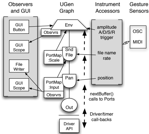
Figure 5: The detailed CSL graph for the sound file player shows the unit generators at the center, the GUI I/O connected via the observer dependency pattern on the left, and the Instrument object's accessors on the right, connected to OSC and MIDI I/O.
