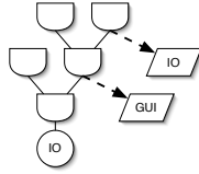
Figure 3: CSL processing graphs are activated by IO objects. Other IO objects or GUI displays then use the Observer/Observable relationship (shown as dotted arrows in the Figure) to attach themselves to any unit generator in the graph.
