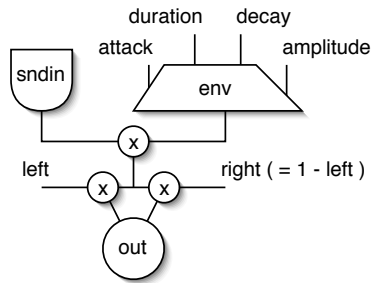
Figure 4: Sound file player instrument graph from the canonical software sound synthesis paper; a sample reader/player object is scaled by an envelope and panner to a stereo output. In CSL (and other modern languages) the graph would use four unit generators.
