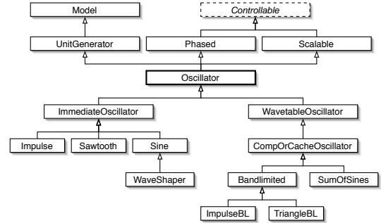
Figure 1: The (partial) class hierarchy of CSL Oscillator UnitGenerators showing multiple inheritance from UnitGenerator , Phased , and Scalable (the last 2 of which are both subclasses of Controllable ). The concrete subclasses each implement (at least) a constructor and a nextBuffer method.
